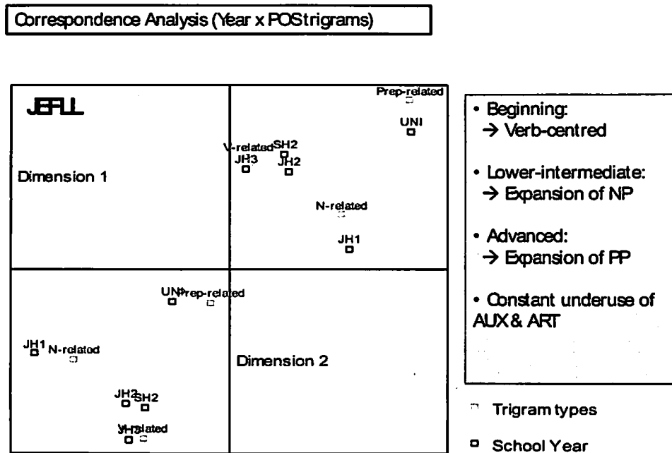
Figure 2. Tono (2000): Analysis of POS tag sequences across proficiency
